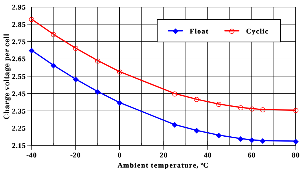
Figure IV: Temperature compensation of charge voltage
