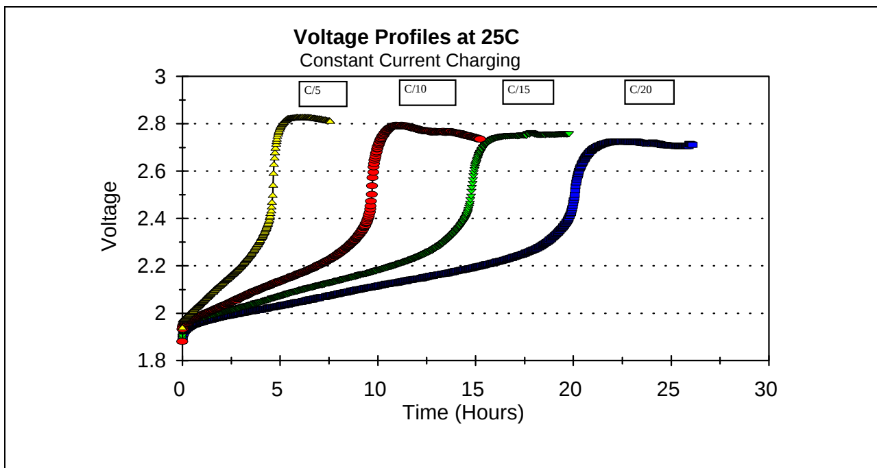
Figure V : Constant current charging at 25°C
