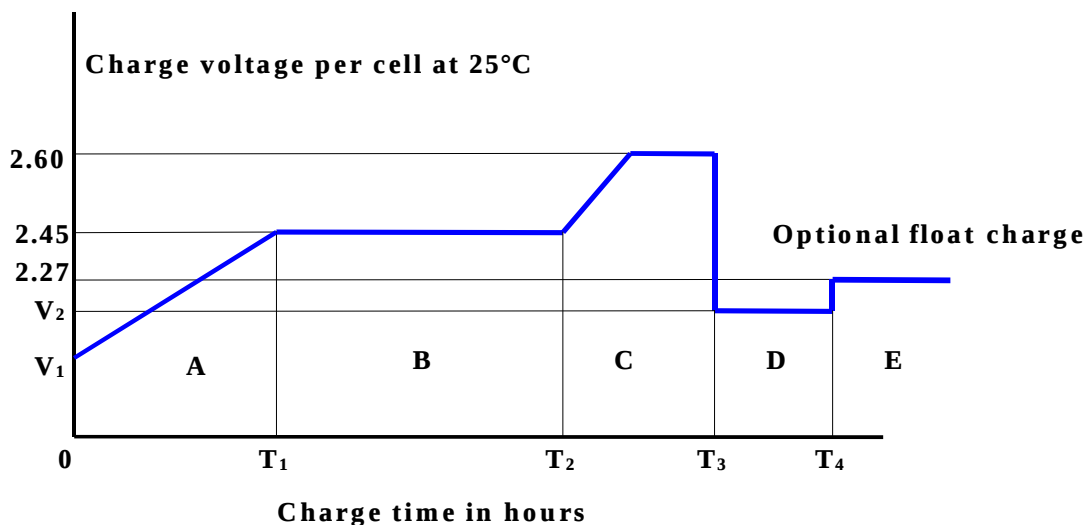
Figure II: Voltage profile under IUI charge (not to scale)
