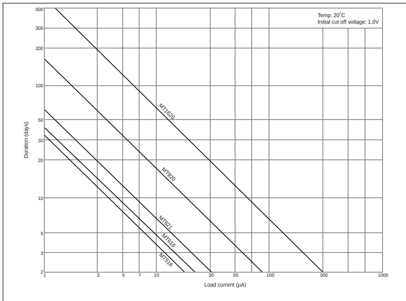
Current drain as a function of duration
