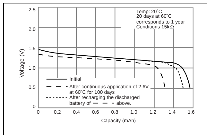
Storage characteristics (MT621)
