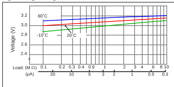
Operating voltage vs. load resistance
