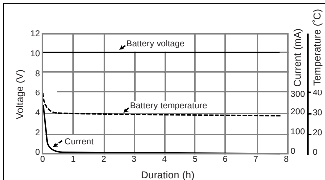
Charge resistance characteristics of BR2325 (10 V consistent-voltage charging)
