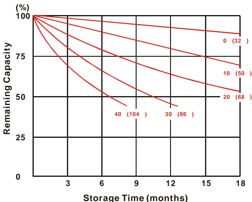
Capacity Retention Characteristic
