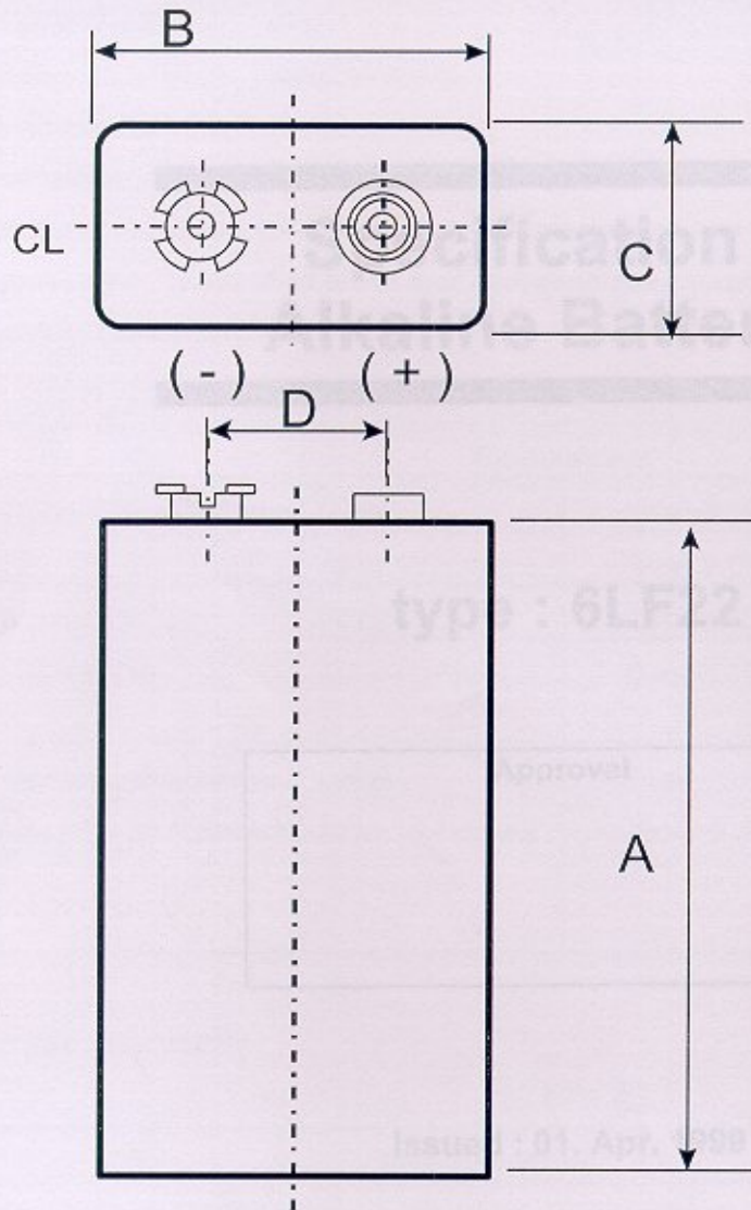
6LF22 Dimension Drawing
