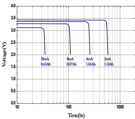
Continuous Discharge at 20°C
