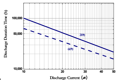
Discharge Current vs. Duration Time
