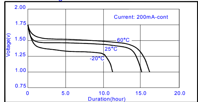
Discharge Characteristics
