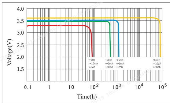
Typical discharge curves at 23°C
