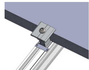
Inter Clamp
