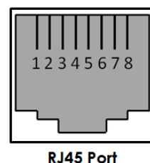
RJ45 Port
