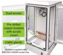
PCE compartment with 3 door access.
