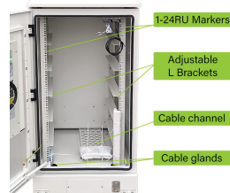
Adjustable height shelves for different modules.
