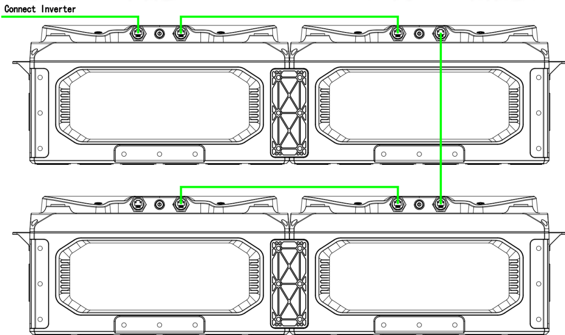
Figure 5-7: Connecting the communication port between parallel voltgo batteries.
