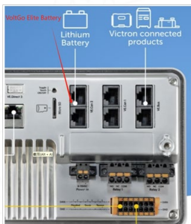
Figure 5-6: Victron Energy Ekrano GX VE Con port and Voltgo Elite series battery CAN port
