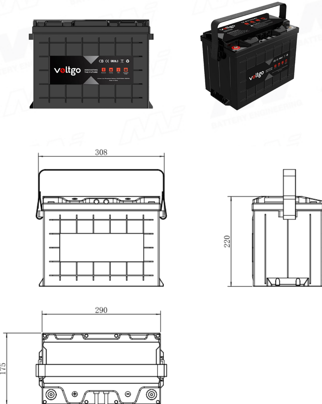
Figure 4-1: VLRV1280 Series Appearance drawing
