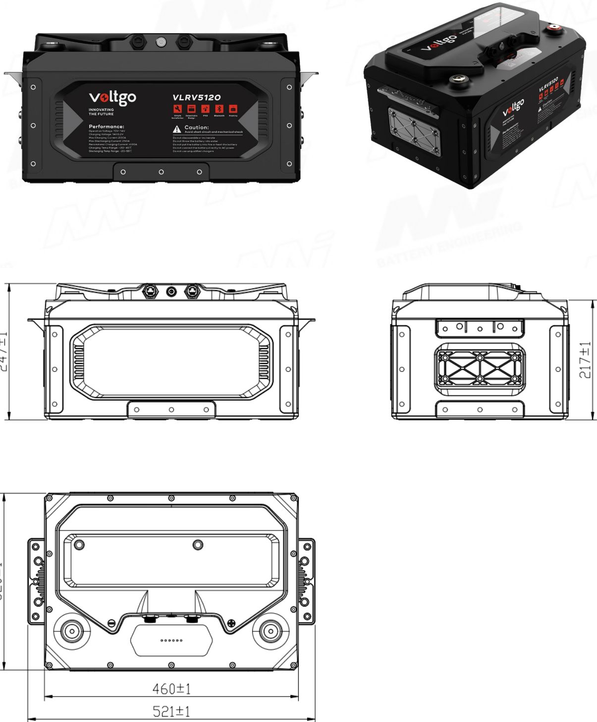
Figure 4-3: VLRV5120 Series Appearance drawing
