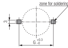
layout top view
