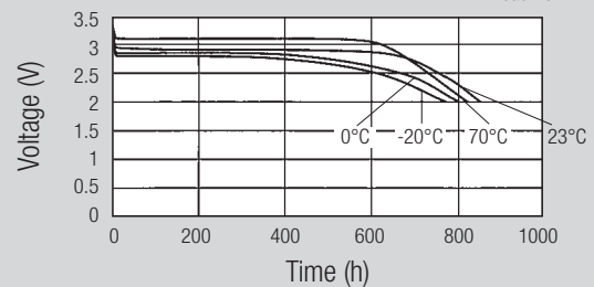
Temperature performance Load 16.2 kΩ
