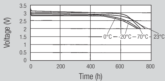
Temperature performance Load 27 kΩ
